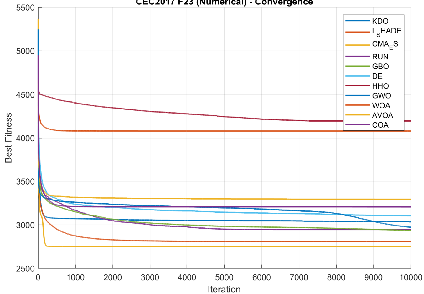
CEC2017 F23 (Numerical) - Convergence
